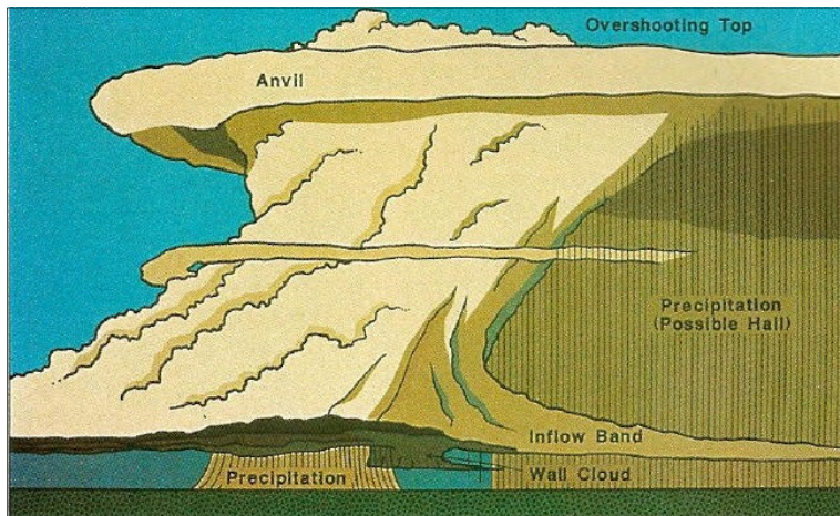
Schematic of a High Precipitation Supercell
